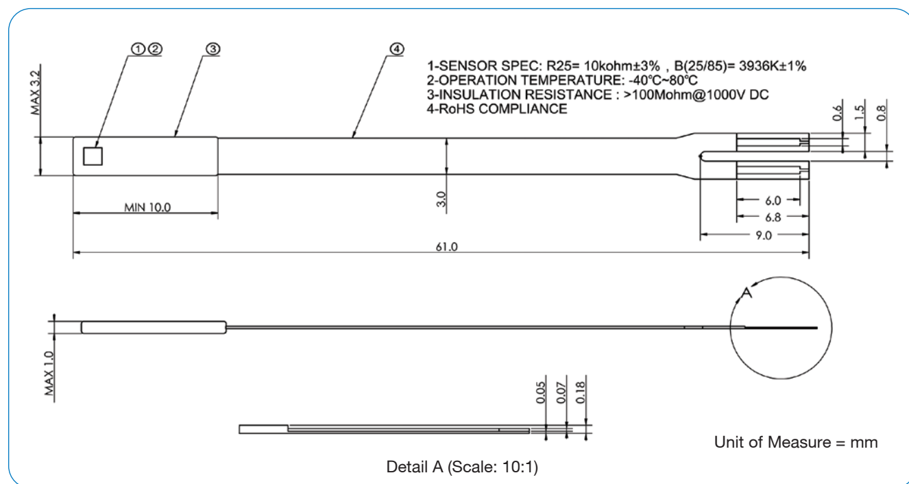
CTTS-203856-S02 Dimensions
