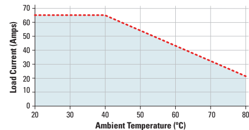
HS072 w/90 Amps single channel SSR
