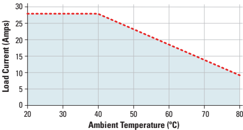
HS251 w/50 Amps single channel SSR
