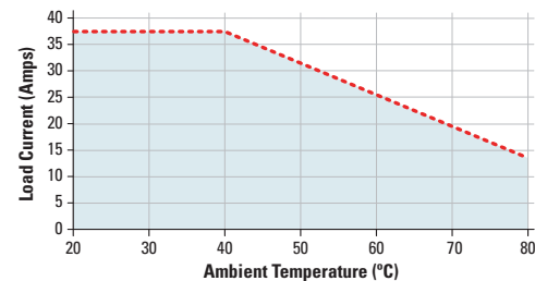
HS172 w/50 Amps single channel SSR
