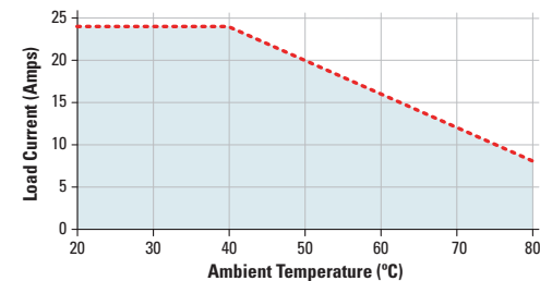
HS301DR w/25 Amps single channel SSR
