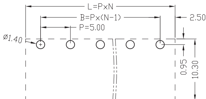
PCB LAYOUT
