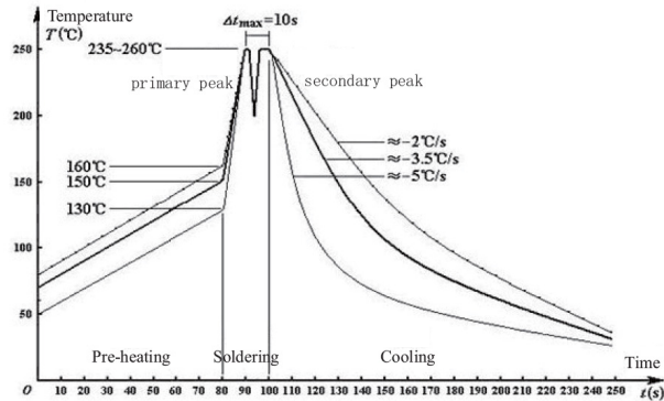
Double-wave Soldering Curve
