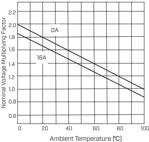
Operating Range
