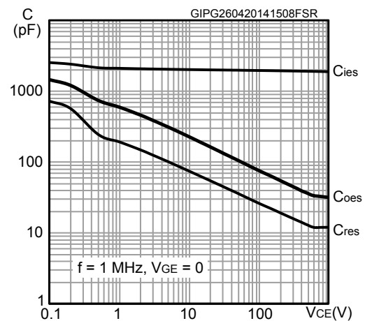
Figure 12. Capacitance variations
