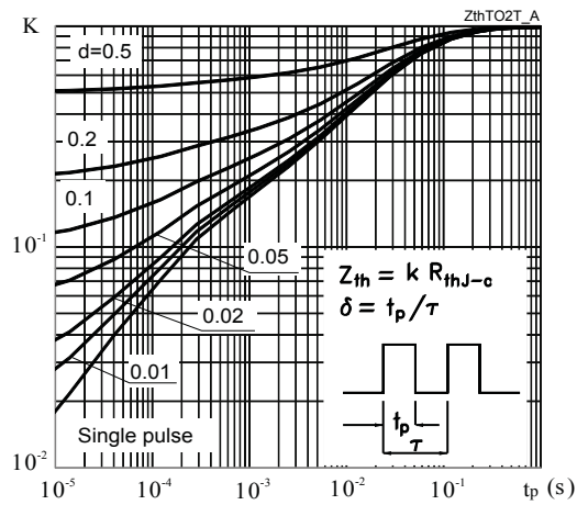
Figure 25. Thermal impedance for IGBT
