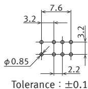
Recommended PC board pattern (BOTTOM VIEW)
