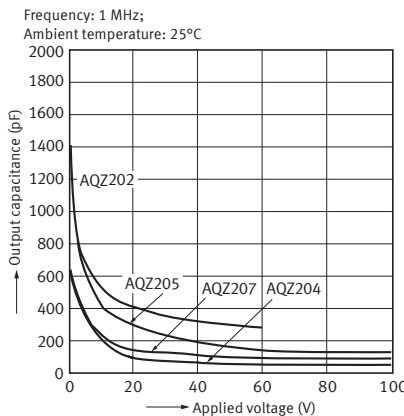
18-2. Output capacitance vs. applied voltage characteristics ( AC/DC type )
