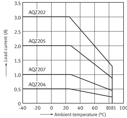
1-2. Load current vs. ambient temperature characteristics ( AC/DC type )
