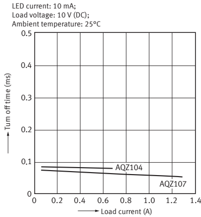
16-2. Turn off time vs. load current characteristics ( DC type )
