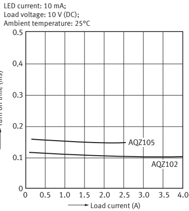
16-1. Turn off time vs. load current characteristics ( DC type )
