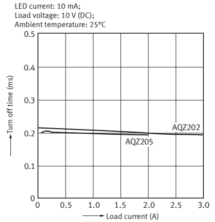
16-3. Turn off time vs. load current characteristics ( AC/DC type )
