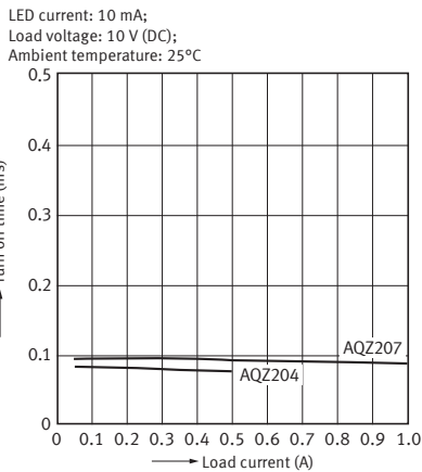
16-4. Turn off time vs. load current characteristics ( AC/DC type )
