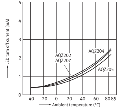
7-2. LED turn off current vs. ambient temperature characteristics ( AC/DC type )
