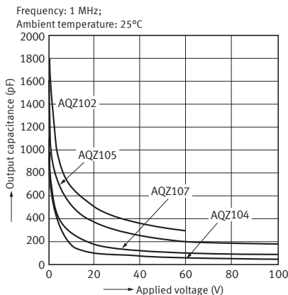
18-1. Output capacitance vs. applied voltage characteristics ( DC type )
