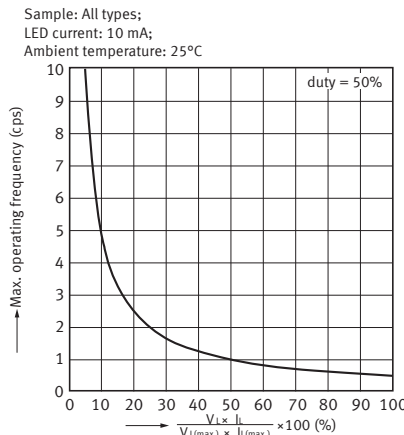
17. Max. operating frequency vs. load voltage and load current
