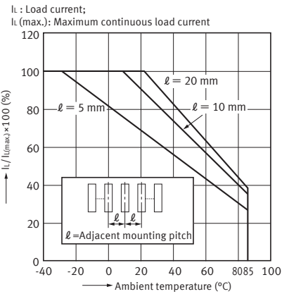
2. Load current vs. ambient temperature characteristics in adjacent mounting
