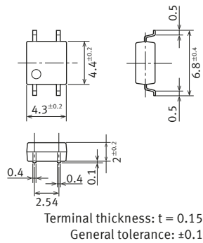
External dimensions
