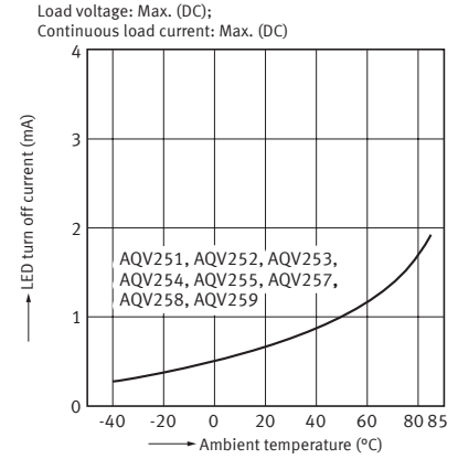
6-1. LED turn off current vs. ambient temperature characteristics
