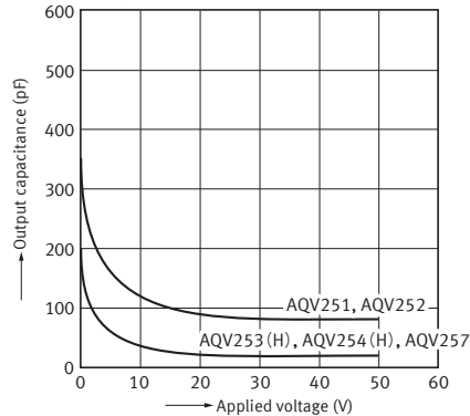
12-1. Output capacitance vs. applied voltage characteristics
