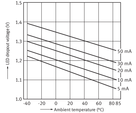
7-1. LED dropout voltage vs. ambient temperature characteristics
