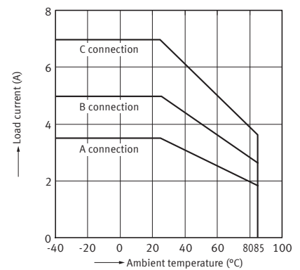
1-3. Load current vs. ambient temperature characteristics
