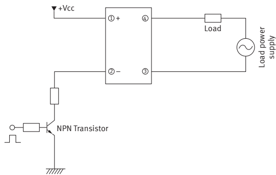
( 1 ) Phototriac Coupler
