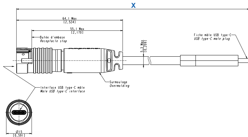
Push-pull version
