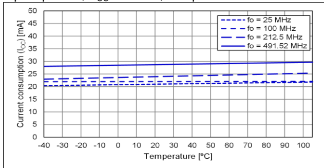
Output option:A, V_{CC} = 2.25 \text{ V} , Temp. Characteristic
