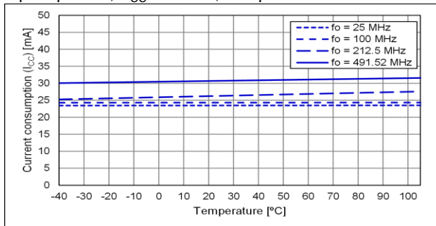
Output option:B, V_{CC} = 2.25 \text{ V} , Temp. Characteristic
