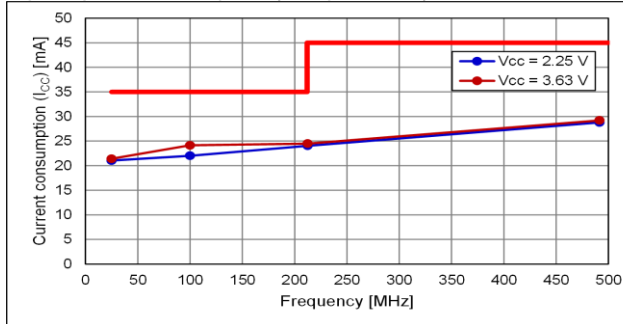
Output option:A, Frequency Dependency
