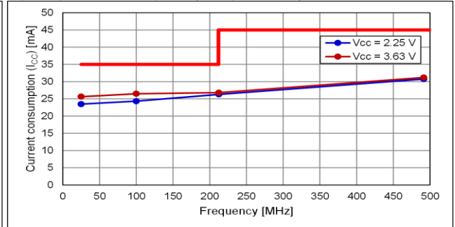
Output option:B, Frequency Dependency
