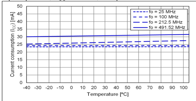
Output option:B, V_{CC} = 2.25 \text{ V} , Temp. Characteristic
