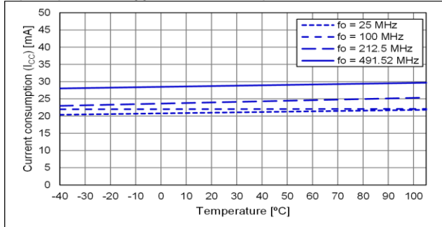
Output option:A, V_{CC} = 2.25 \text{ V} , Temp. Characteristic
