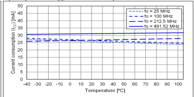
Output option:B, V_{CC} = 3.63 \text{ V} , Temp. Characteristic
