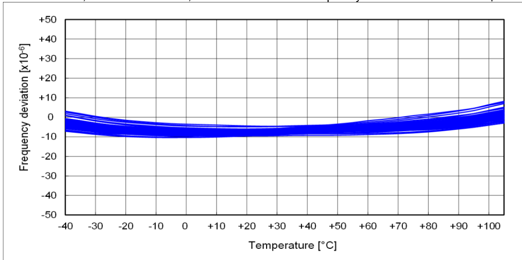
Output option:A, Frequency Dependency
