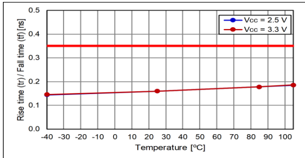
Rise Time
