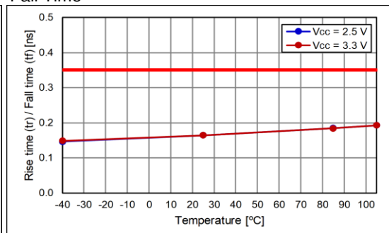
Fall Time
