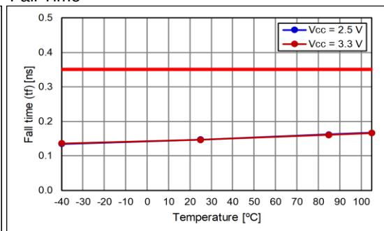
Fall Time
