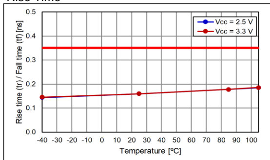
Rise Time
