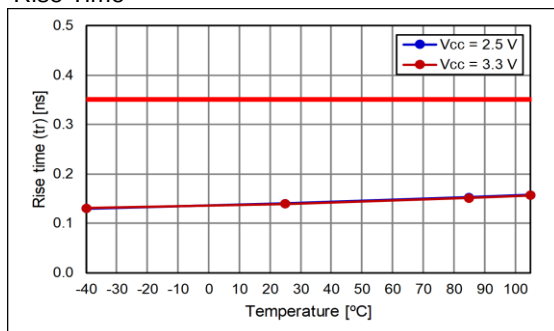
Rise Time
