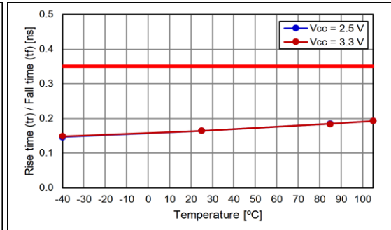
Fall Time
