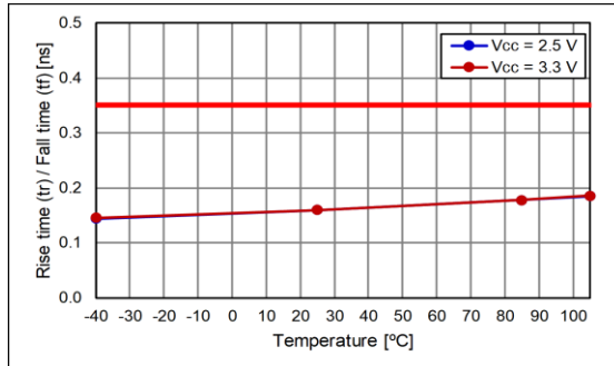
Rise Time
