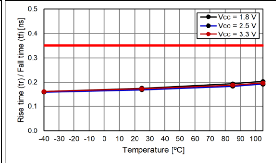
Fall Time
