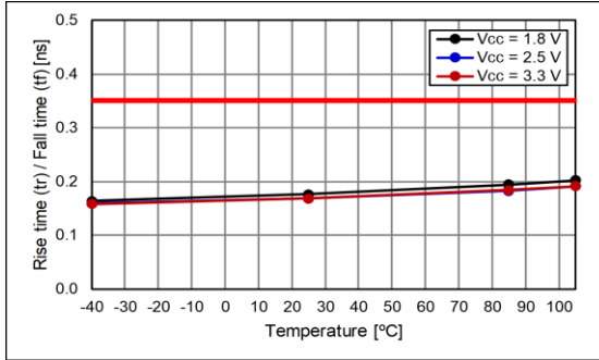
Rise Time
