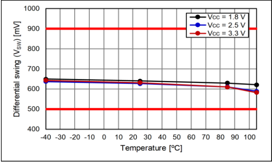
(7-6) Differential Swing Temperature Characteristic fo = 156.25 MHz
