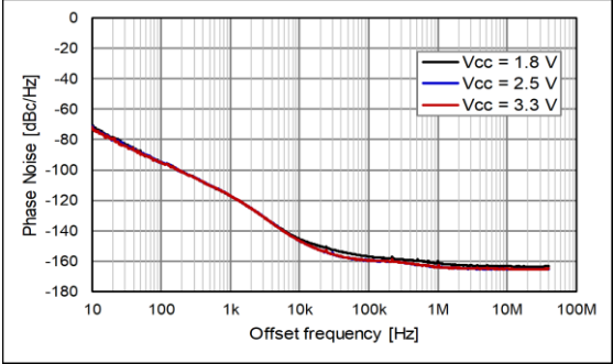
(7-7) Phase Noise and Phase Jitter fo = 156.25 MHz, T use = +25 °C
