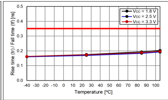
Fall Time
