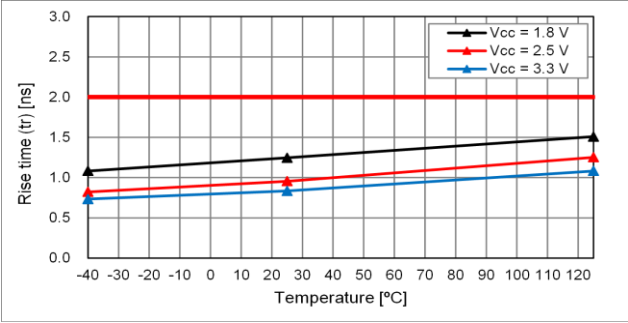
(7-3) Rise/Fall Time [cont'd] Temperature Characteristic (20 % - 80 %V CC , L CMOS = 15 pF) fo = 150 MHz, Rise/Fall time: A (Default) or B (Faster)
