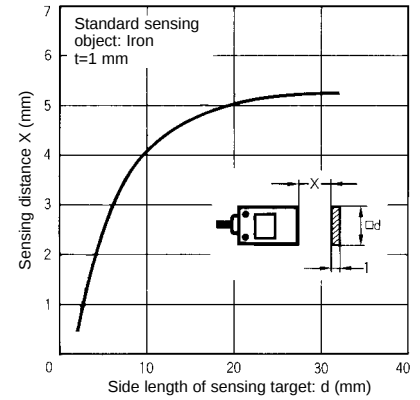
TL-Q5MC□ (Rectangular Model)
