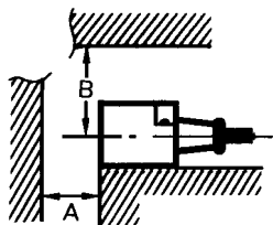
Minimum Distances for Surrounding Metals
