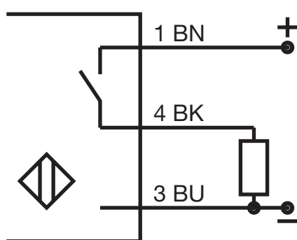
Fig. 10 PNP - Normally open
