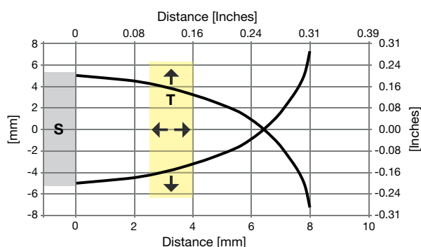
Fig. 2 M12 Non-flush
