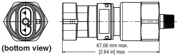
Figure 8. AMP Superseal 1.5
