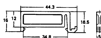
PFP-S Spacer
