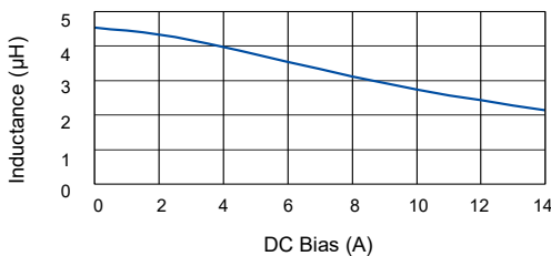
[ ETQP4M4R7YFP ]
