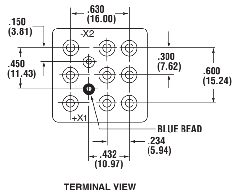
TERMINAL VIEW
