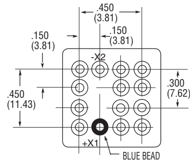
TERMINAL VIEW
