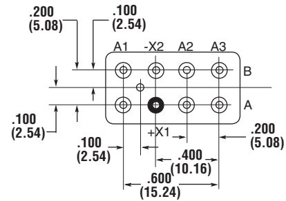
TERMINAL VIEW
