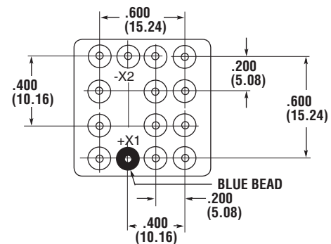
TERMINAL VIEW
