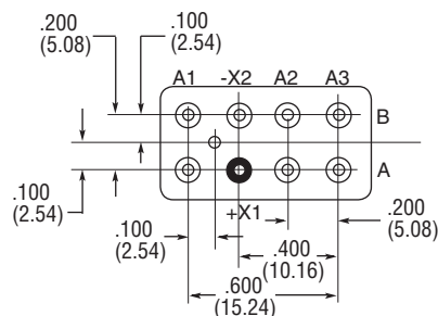
TERMINAL VIEW
