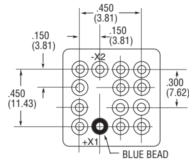
TERMINAL VIEW
