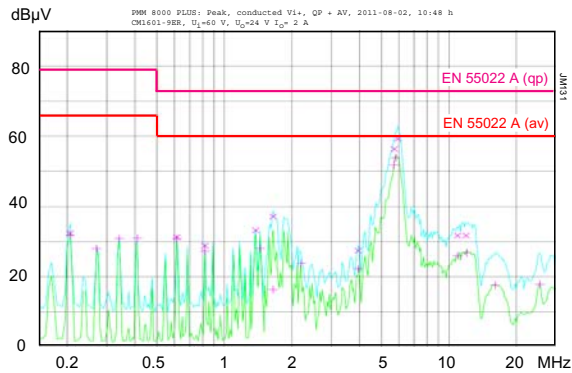
Fig. 13a Typ. conducted disturbances at the input (quasi-peak and average) of CM1601-9ER according to IEC/EN 55011/22, measured at V_i = 60 VDC and I_{o\ nom} .
