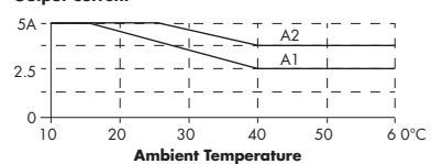
Output Current
