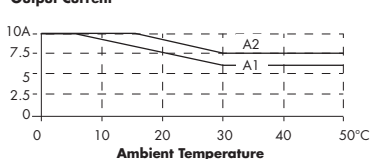
Output Current
