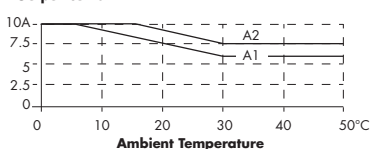
Output Current
