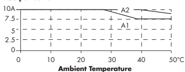
Output Current
