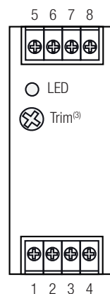
Pin Connections
