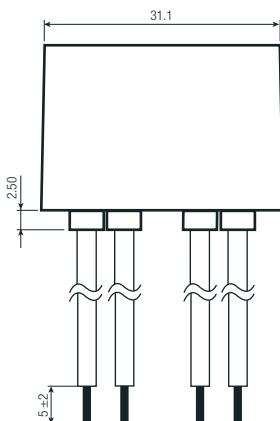
Wired information
