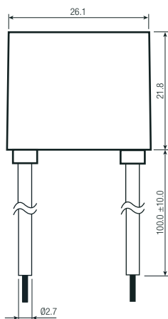
Dimension Drawing Wired (mm)
