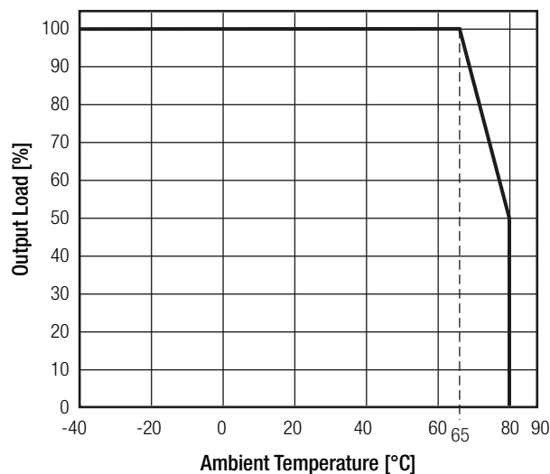
RAC04-xxS(D)C/277-E
