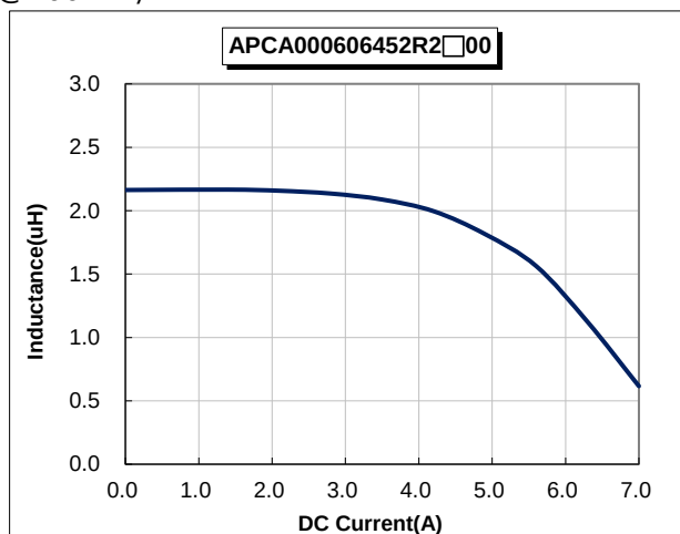
INDUCTANCE vs. DC CURRENT @100kHz/1V
