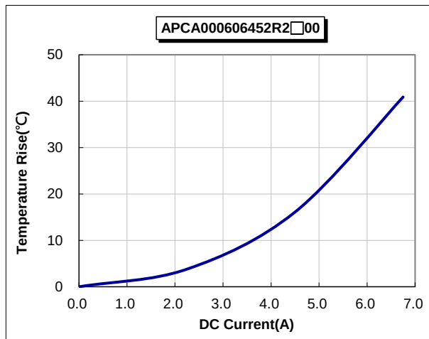
TEMPERATURE vs. DC CURRENT
