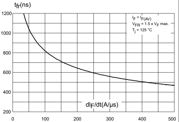
Figure 10. Forward recovery times versus dl_F/dt (typical values)
