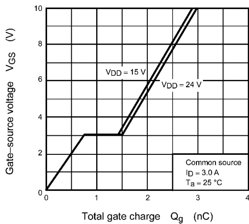
Fig. 9.9 Dynamic Input/Output Characteristics
