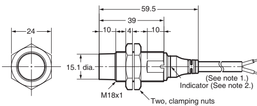
E2A-S18KN16-WP-□
