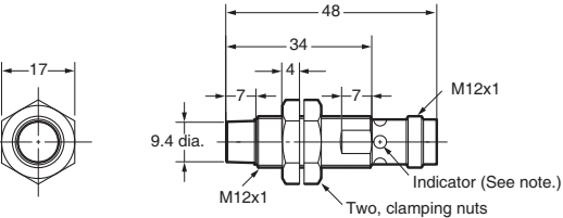
E2A-S12KN08-M1-□
