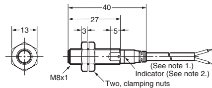
E2A-S08KS02-WP-□□
