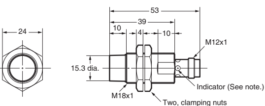
E2A-S18KN16-M1-□
