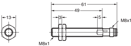
E2A-S08LS02-M5-□□/E2A-S08LS02-M3-□
