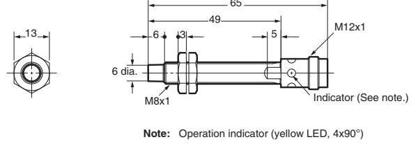
E2A-S08LN04-M1-□□
