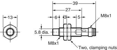
E2A-S08KN04-M5-□□/E2A-S08KN04-M3-□
