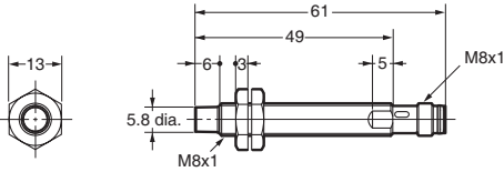
E2A-S08LN04-M5-□□/E2A-S08LN04-M3-□
