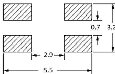
Recommended Layout
