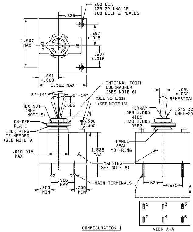
FIGURE 1. Circuit breaker configuration.
