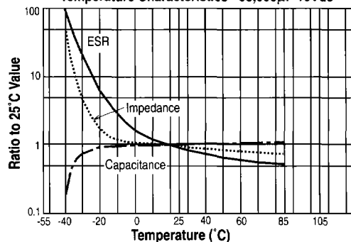
Temperature Characteristics - 98,000 \mu F 10Vdc
