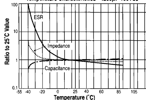
Temperature Characteristics - 4200 \mu F 100Vdc
