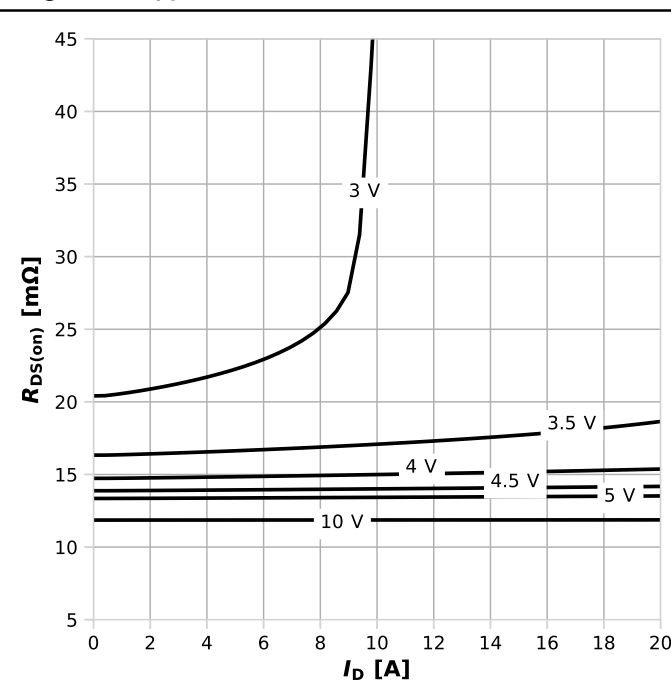
Diagram 6: Typ. drain-source on resistance (n-channel)
