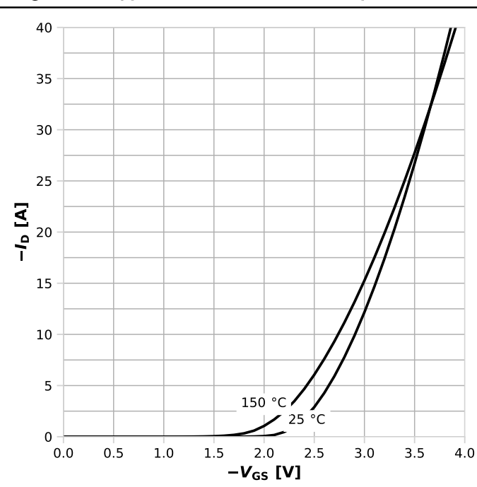
Diagram 22: Typ. transfer characteristics (p-channel)
