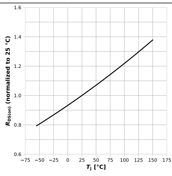
Diagram 24: Normalized drain-source on resistance (p-ch.)
