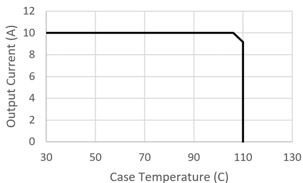
i1C4W010A120V-xxx-R
