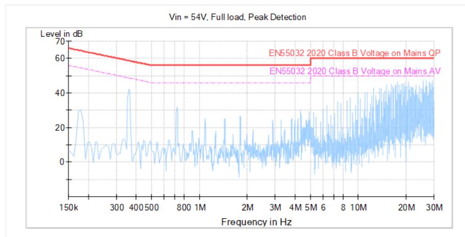
Conducted Emissions Performance, Negative Line CISPR 22, Class B, full load
