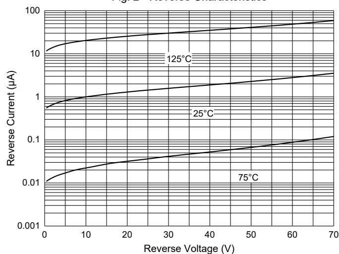
Fig. 2 - Reverse Characteristics
