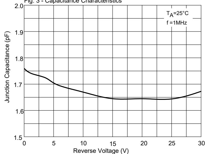
Fig. 3 - Capacitance Characteristics
