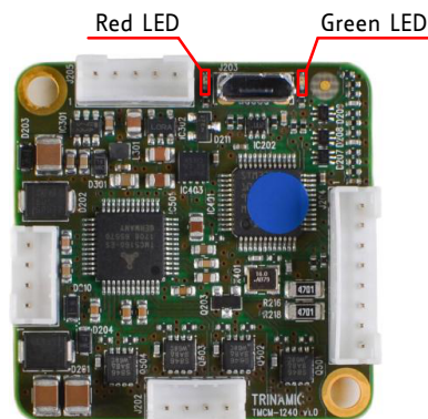
Figure 3: TMCM-1240 LEDs
