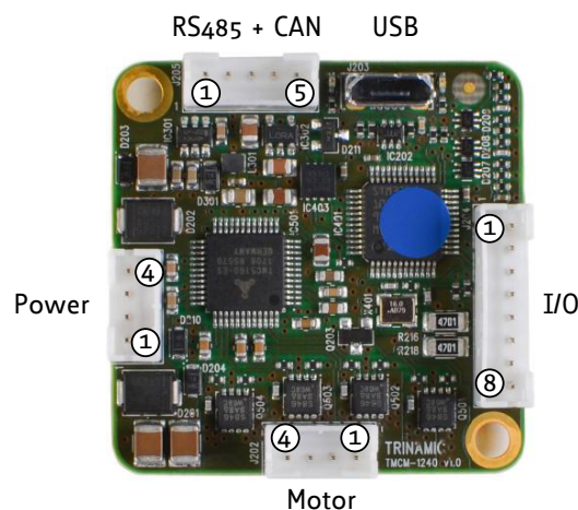
Figure 2: TCM-1240 connectors
