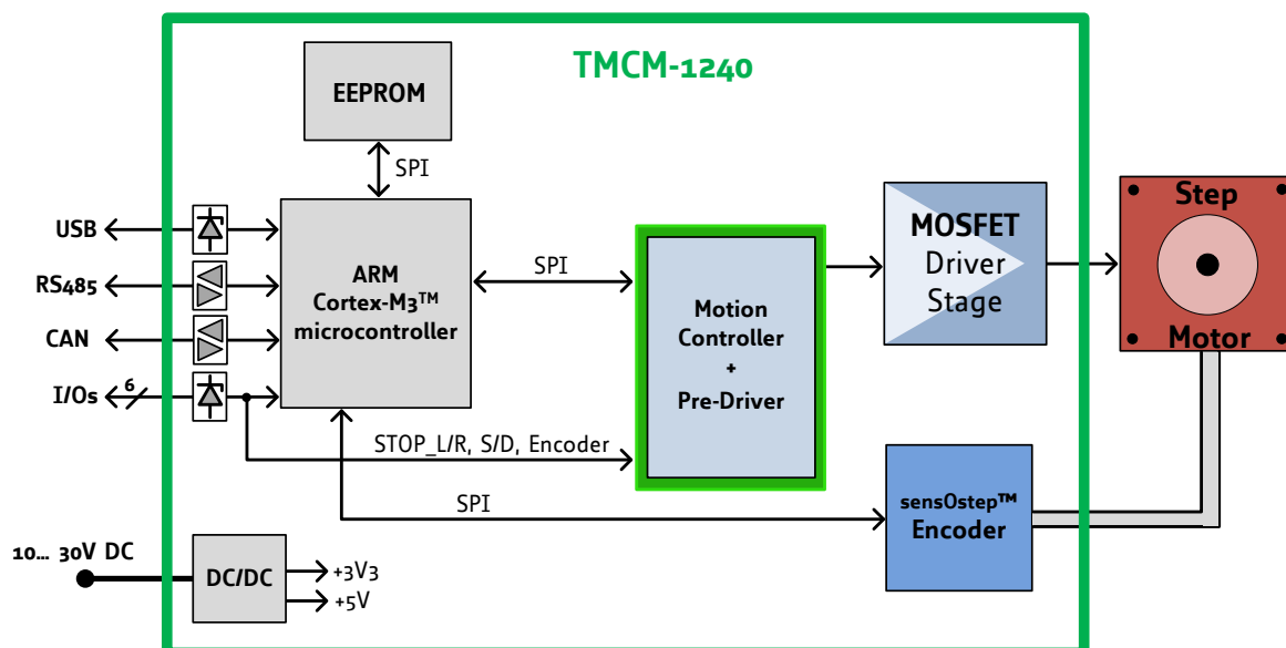
Figure 14: TMC1240 block diagram
