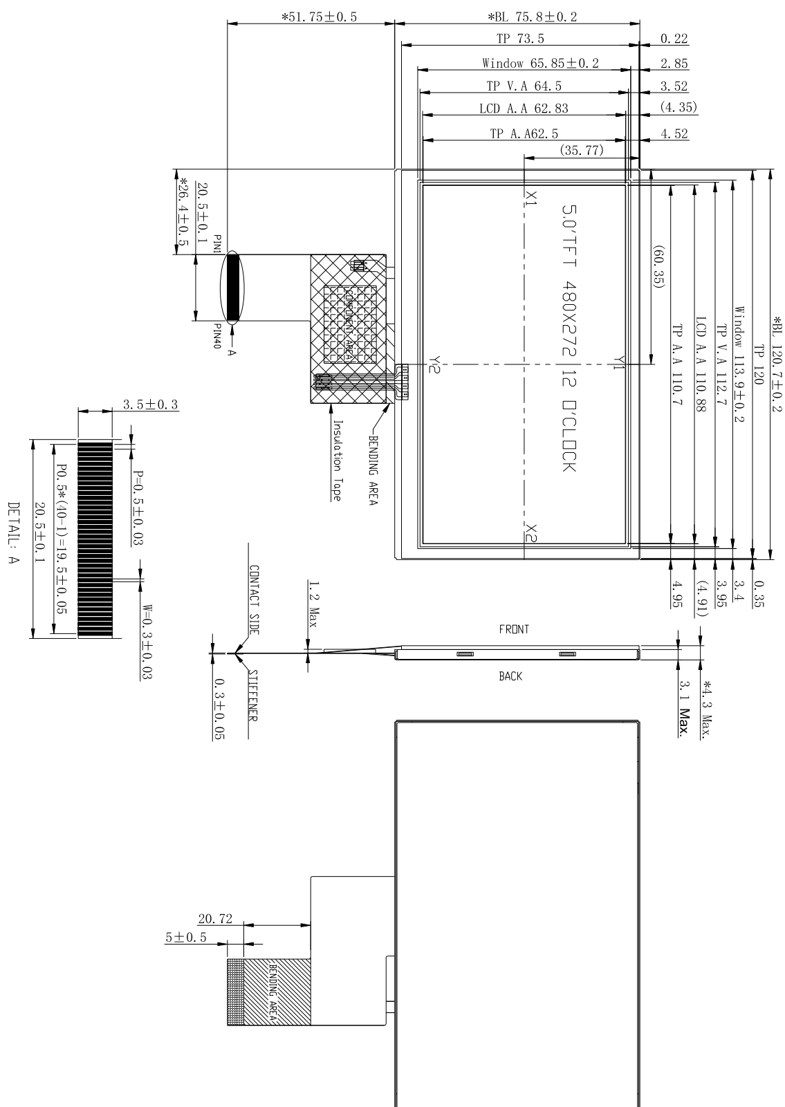
Figure 11 - LCM Dimension
