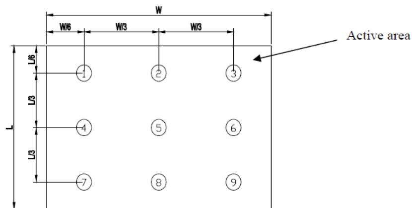
Figure 4 - Measurement Point
