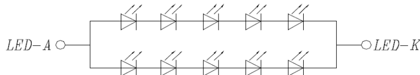
Figure 2 - Backlight LED Circuit
